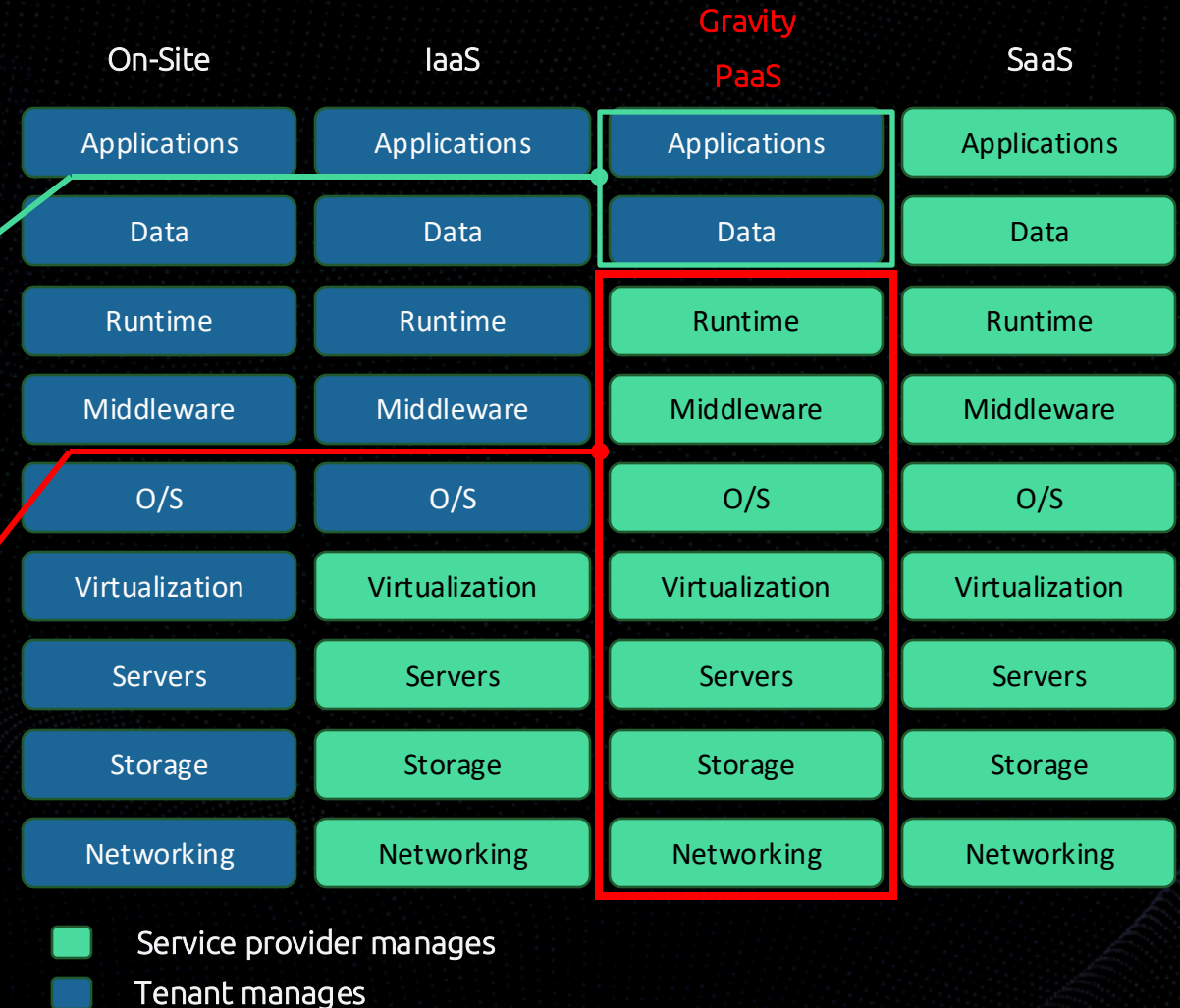
Shared Responsibility Model
